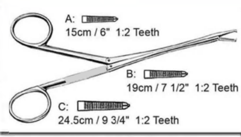
50-554-00 A / B / C Brand Tendon Tunnelling Forceps
