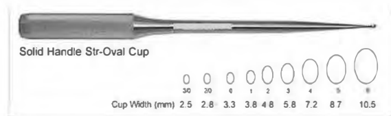
50-442-28 Spinal Fusion Curette 28 cm / 11"
