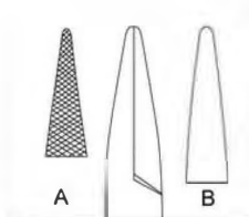
50-223-14 Needle Nose Pliers Taper to 2mm Tip 14 cm / 5 1/2" A: Fine Cross Serration B: Smooth
