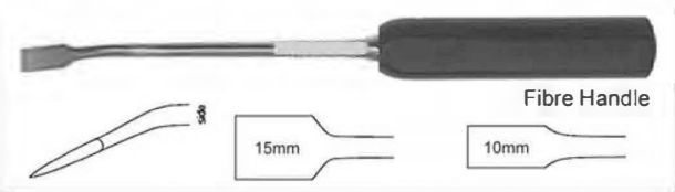
50-406-00 Lexer Osteotome Angled / 28cm/11"
