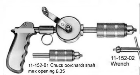
50-157-00 Martin Hand Drill with Chuck & Wrench
