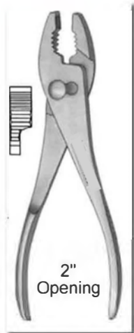
2" Opening 50-239-20 20 cm / 8" Slip Joint Pliers
